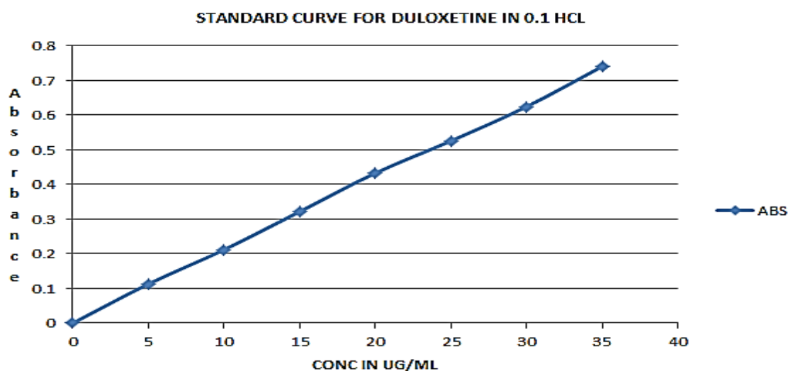
Figure 1. UV spectrophotometric calibration curve of duloxetine hydrochloride (288 nm)
