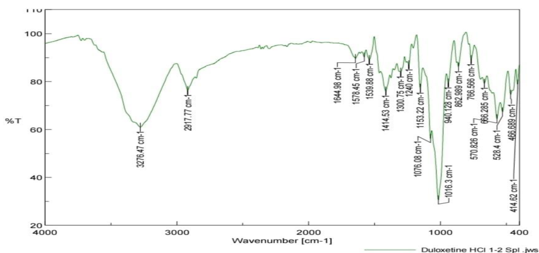
Figure 2. FTIR spectrum of the duloxetine hydrochloride- \beta -cyclodextrin inclusion complex (1:2)
