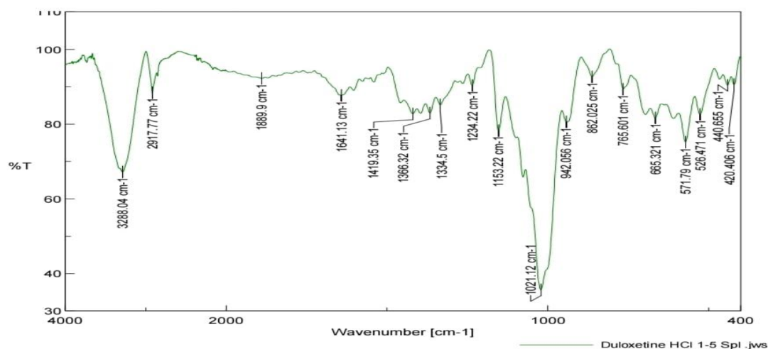
Figure 3. FTIR spectrum of the duloxetine hydrochloride- \beta -cyclodextrin inclusion complex (1:5)
