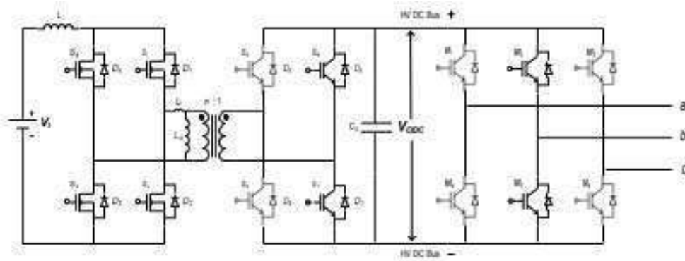
Fig. 7. Energy conversion system with dc-dc converter followed by 3 phase VSI
